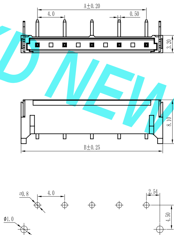
P. C. B LAYOUT
