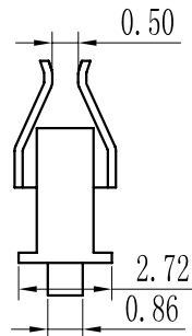
SECTION C-C
