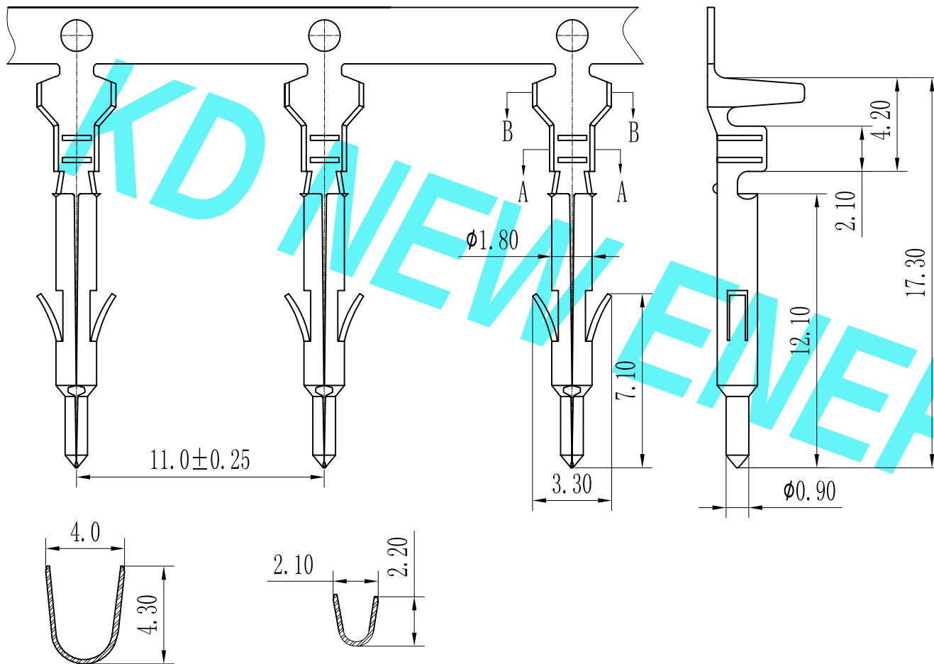
Section: A-A
