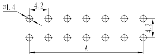
P. C. B LAYOUT
