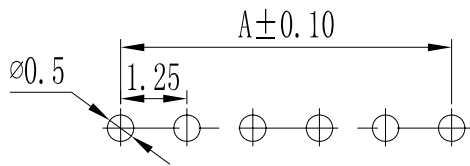
P. C. B LAYOUT
