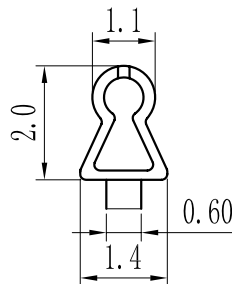
Section: C-C
