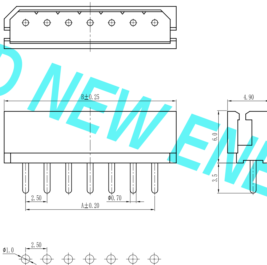
P. C. B LAYOUT
