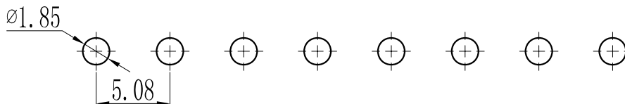
PCB LAYOUT
