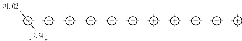
PCB LAYOUT
