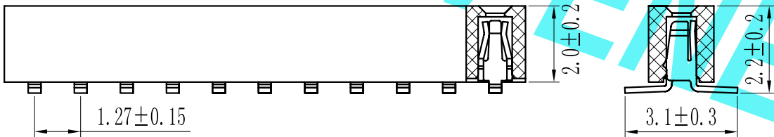
PCB LAYOUT
