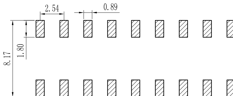
PCB LAYOUT
