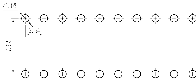
PCB LAYOUT
