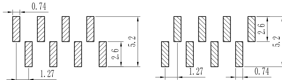
PCB LAYOUT
