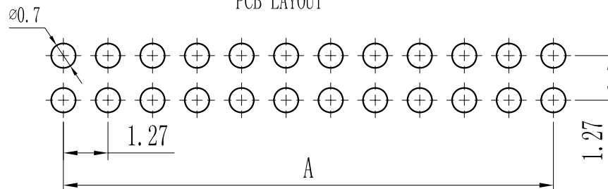
PCB LAYOUT
