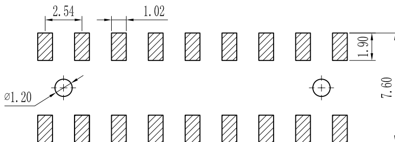
PCB LAYOUT
