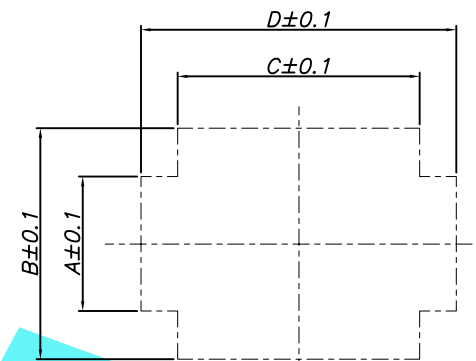
Panel layout
