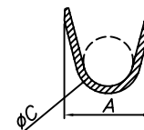
SECTION Z-Z SCALE 10:1 INSULATION GRIP
