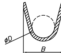
SECTION Y-Y SCALE 10:1 INSULATION GRIP
