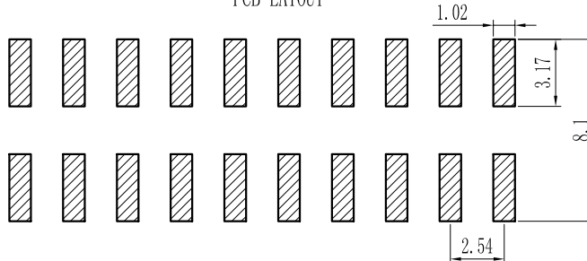
PCB LAYOUT
