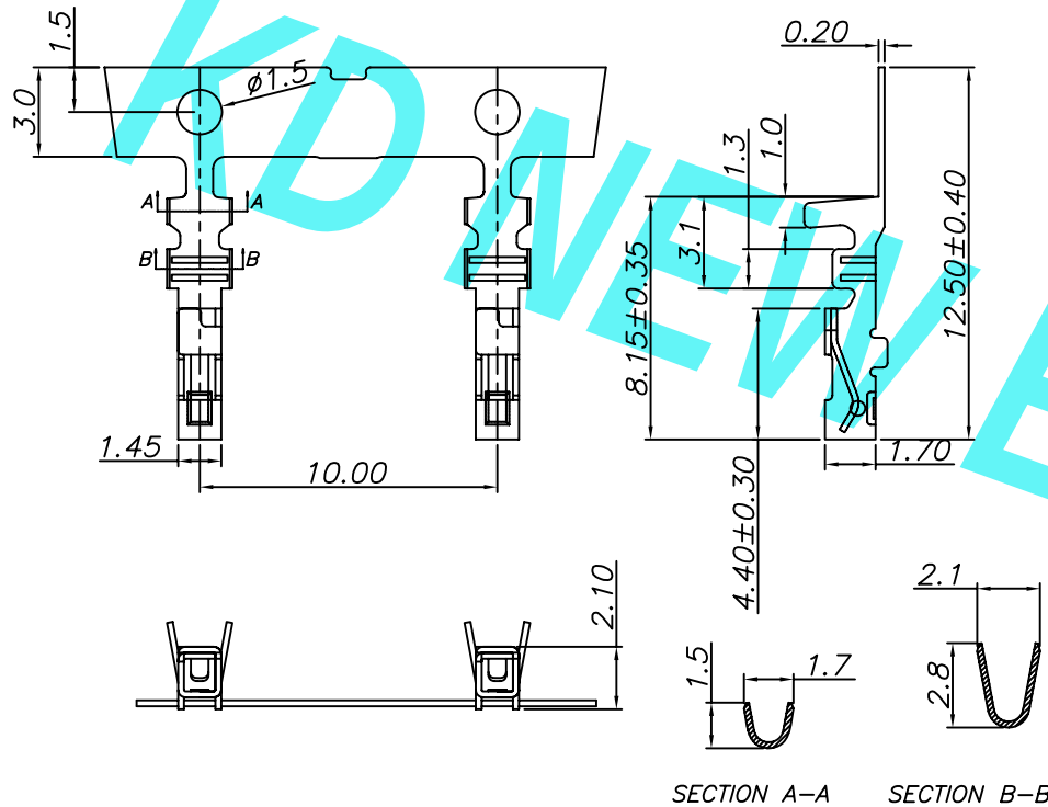
SECTION A-A SECTION B-B
